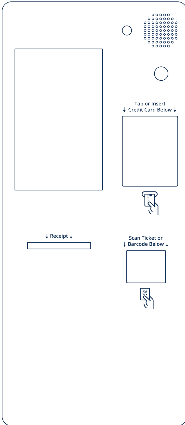
Central Pay-on-Foot — Credit Card Only 1:35 Scale Layout
