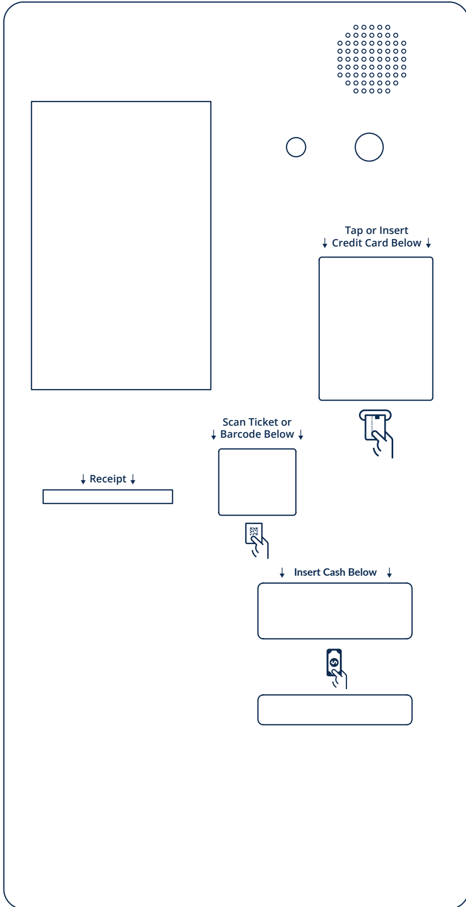
Central Pay-on-Foot — Cash and Credit Card 1:35 Scale Layout
