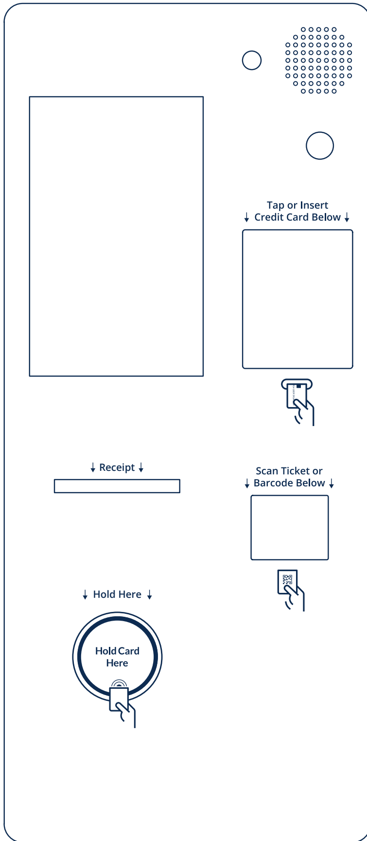
Exit Terminal — With Credit Card 1:35 Scale Layout
